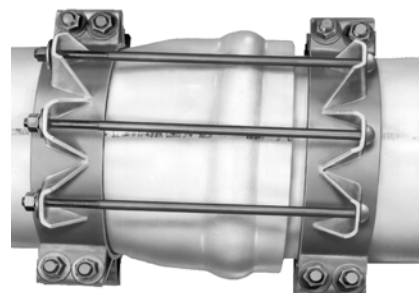
JCM 621 Bell Joint Restrainer
