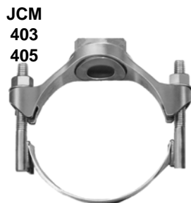
JCM 403/405 Strap Service Saddles with outlets 1-1/4" - 2-1/2"
